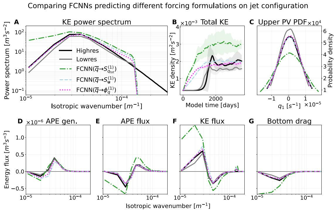
Figure D6. Like Figure 19, but comparing the online jet configuration performance of FCNNs trained to predict different subgrid forcing formulations ( S_{q_{tot}}^{(1)} , S_u^{(1)} , and \phi_q^{(1)} ) computed with Operator 1 (Equation 13). In this case, the models trained to predict S_u^{(1)} and \phi_q^{(1)} appear to generalize better. However, their average scores across the full set of metrics (e.g., Figure D9) remain low, and in KE snapshots from these FCNNs (Figure D3), the characteristic jet behavior we see in high-resolution is absent.
